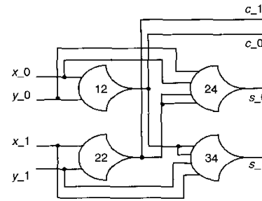
Fig. 2 NCL half-adder
