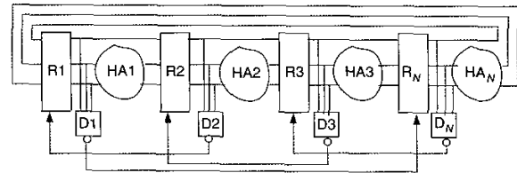
Fig. 3 NCL ring each stage of which is a half-adder
