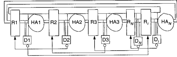
Fig. 6 Ring with initialising stage ( R_i, D_i )
