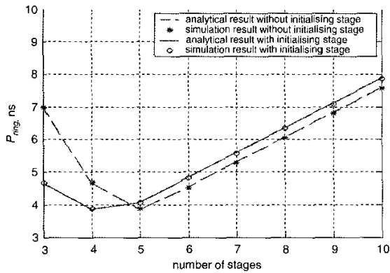
Fig. 7 Circulation period against number of stages
