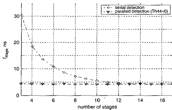
Fig. 11 Simulation results for 24-bit divisions with different completion detection circuit
