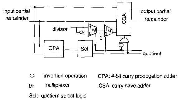
Fig. 9 Combinational logic for one stage of radix-2 SRT division
