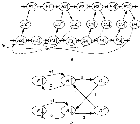
Fig. 5 Dependency graphs for NCL pipeline a Extended dependency graph b Folded dependency graph
