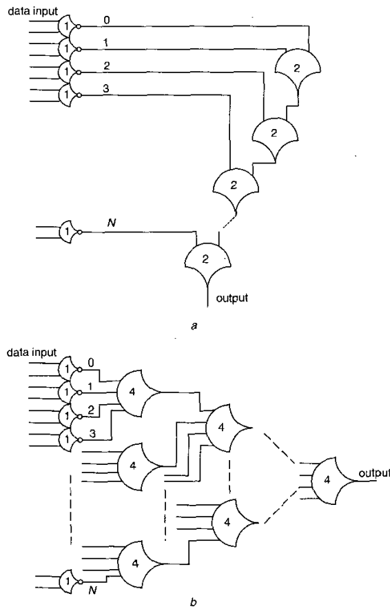
Fig. 10 Completion detection circuits a Serial architecture b Parallel architecture
