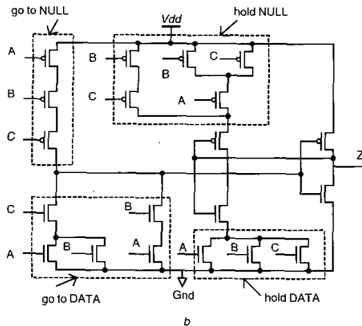
Fig. 1 Threshold gate with hysteresis
