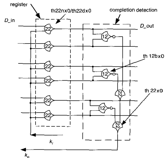
Fig. 4 3-bit register and completion detection
