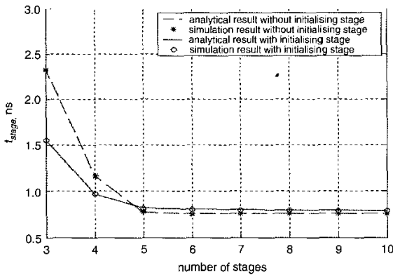
Fig. 8 Per-stage time against number of stages
